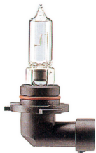
HB 3 White 12V 60W P20d 202570 HB 3 Gold 12V 60W P20d 202587
