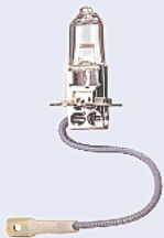
H3 Basic 12V 55W PK22s 202723 H3 +Power 12V 100W PK22s 202730 H3 +Power 12V 130W PK22s 202747
