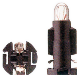
MFL23 Long Life 12V 1,1W 203928
