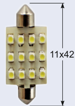
C5W/10W LED 12V 12x3528 T11x42/SV8,5 210179
